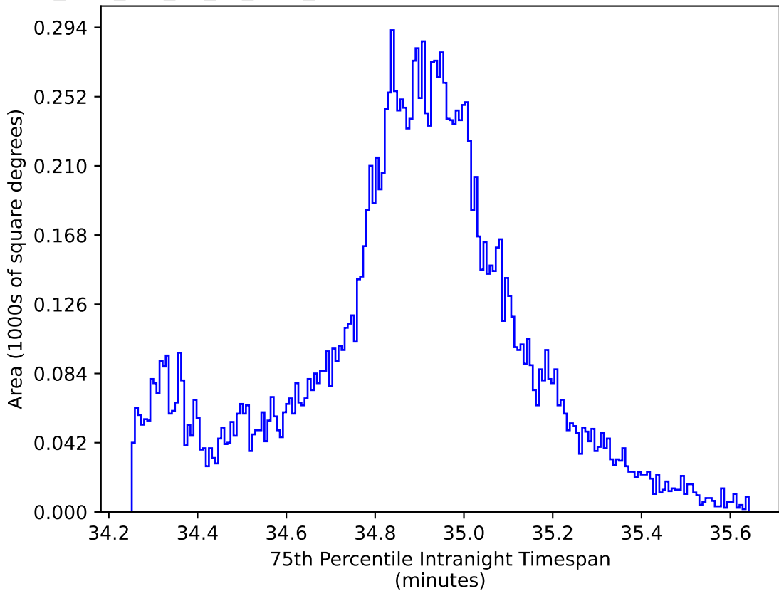
too_elab_r16_d2_gz_v3.4_10yrs WFD: 75th Percentile Intranight Timespan
