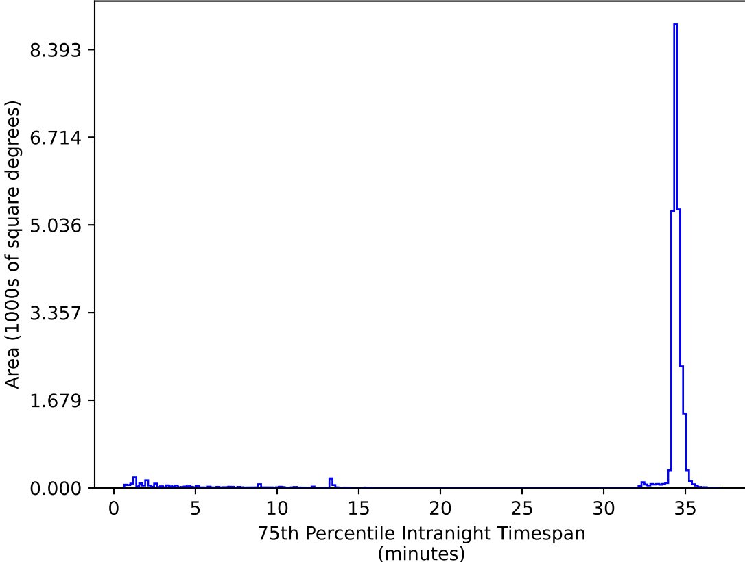
too_elab_r16_d2_gz_v3.4_10yrs All sky zy bands: 75th Percentile Intranight Timespan
