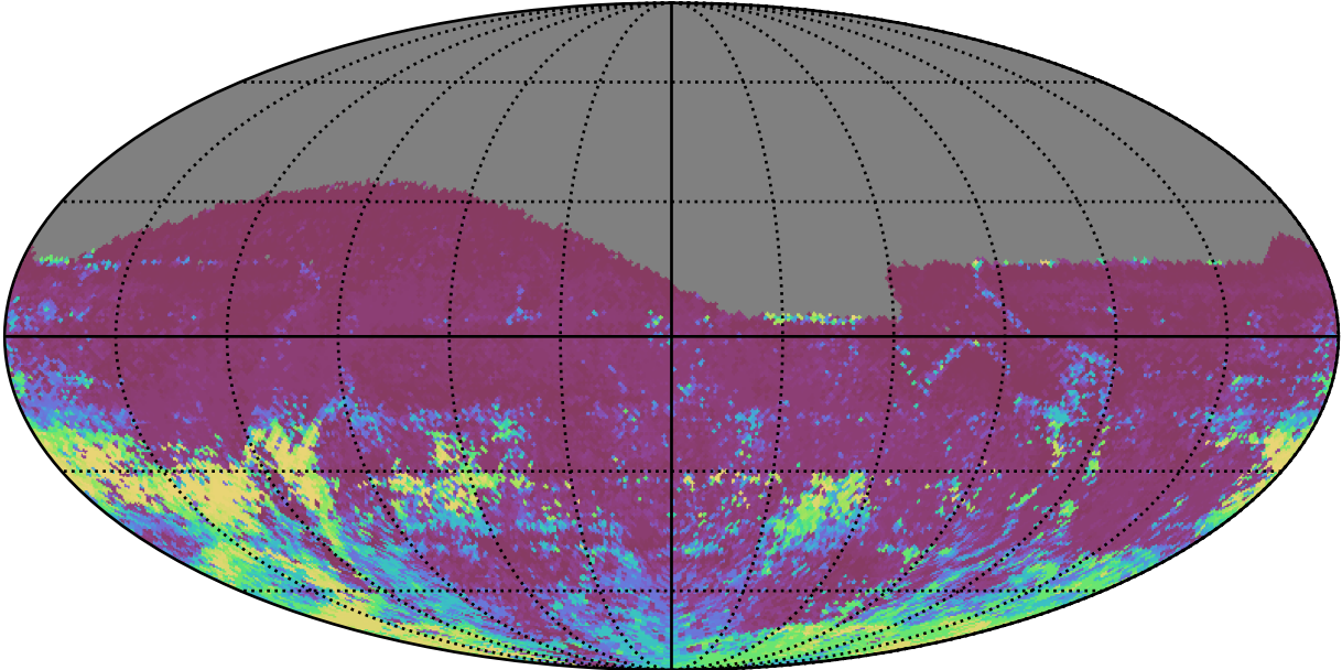
too_elab_r16_d2_gz_v3.4_10yrs All sky r band: 75th Percentile Intranight Timespan
