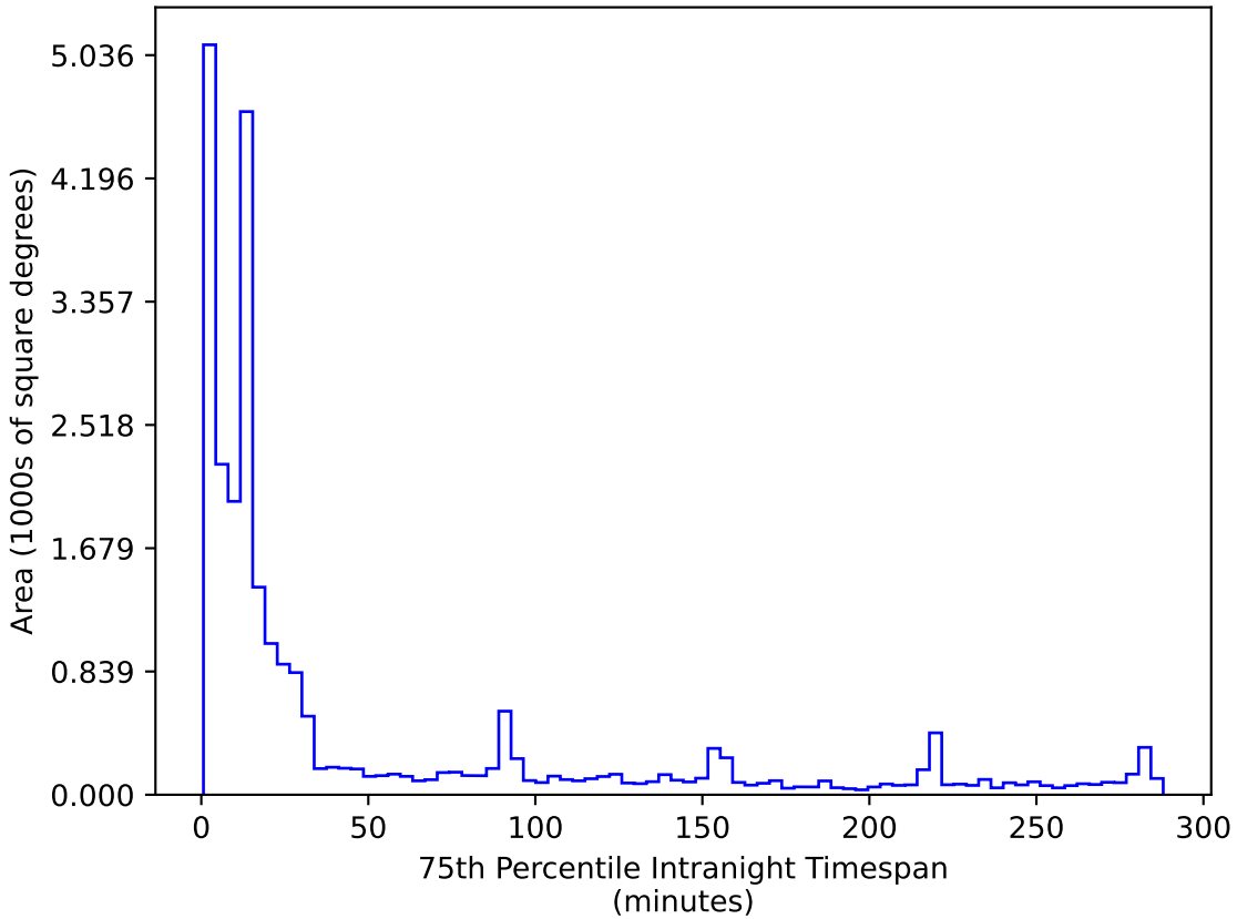
too_elab_r16_d2_gz_v3.4_10yrs All sky r band: 75th Percentile Intranight Timespan
