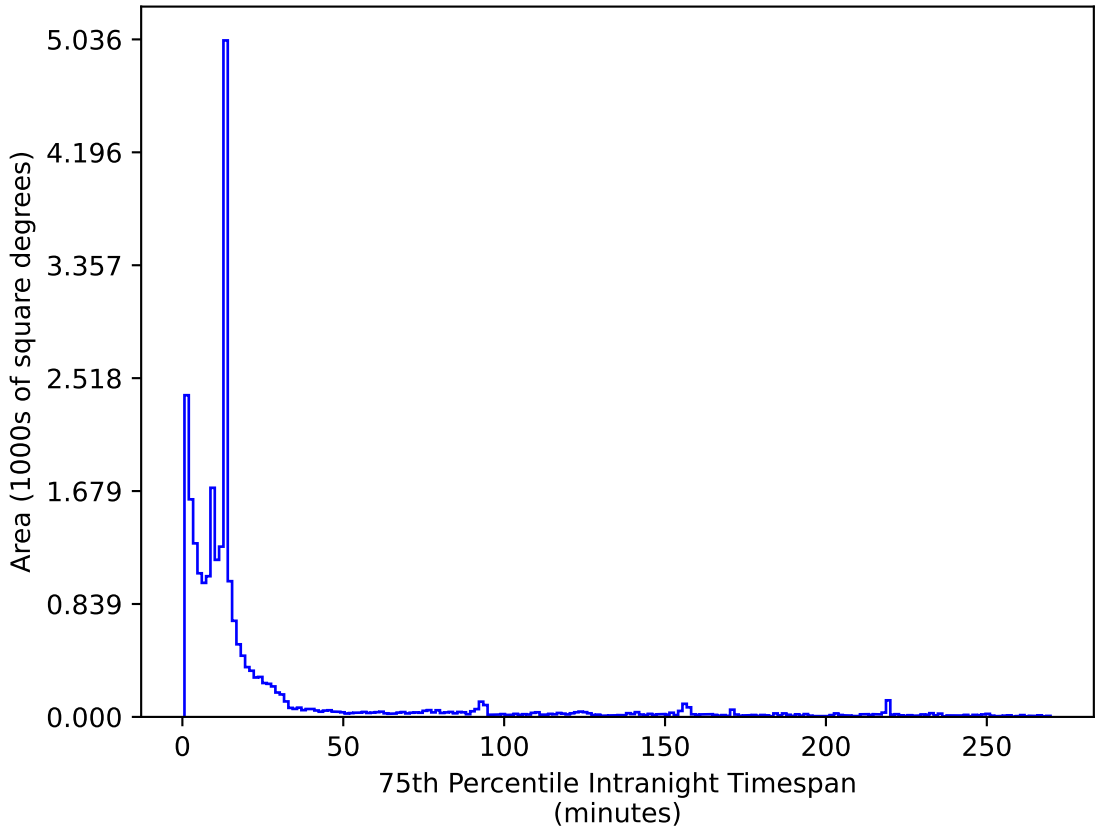
too_elab_r16_d2_gz_v3.4_10yrs All sky i band: 75th Percentile Intranight Timespan
