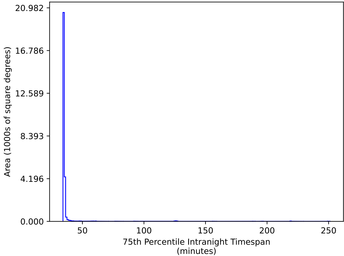
too_elab_r16_d2_gz_v3.4_10yrs All sky gr bands: 75th Percentile Intranight Timespan
