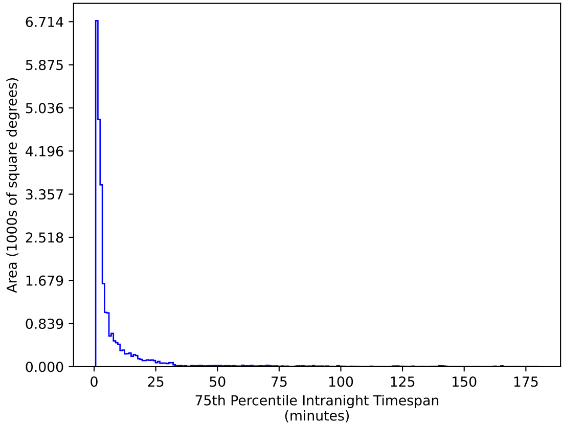
too_elab_r16_d2_gz_v3.4_10yrs All sky g band: 75th Percentile Intranight Timespan
