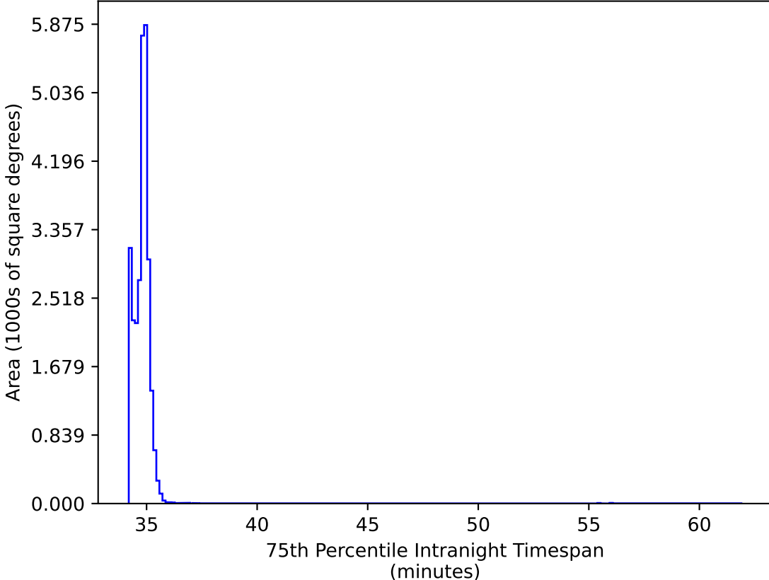
too_elab_r16_d2_gz_v3.4_10yrs All sky all bands: 75th Percentile Intranight Timespan
