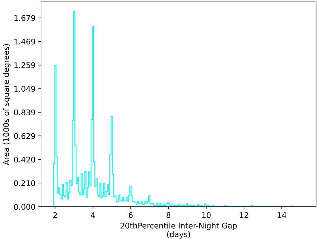
too_elab_r16_d2_gz_v3.4_10yrs WFD u band: 20thPercentile Inter-Night Gap
