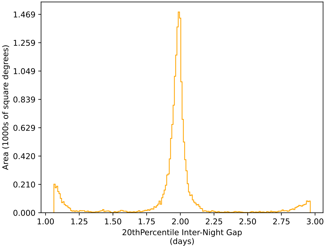
too_elab_r16_d2_gz_v3.4_10yrs WFD r band: 20thPercentile Inter-Night Gap
