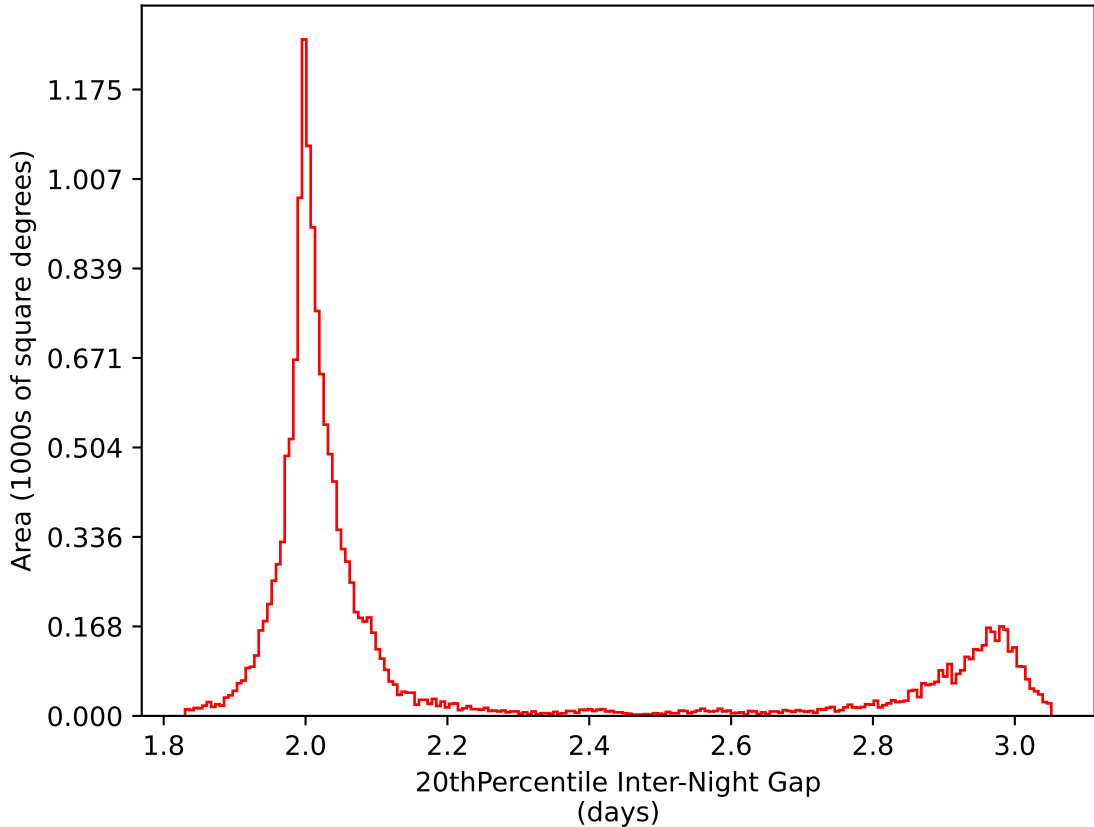
too_elab_r16_d2_gz_v3.4_10yrs WFD i band: 20thPercentile Inter-Night Gap
