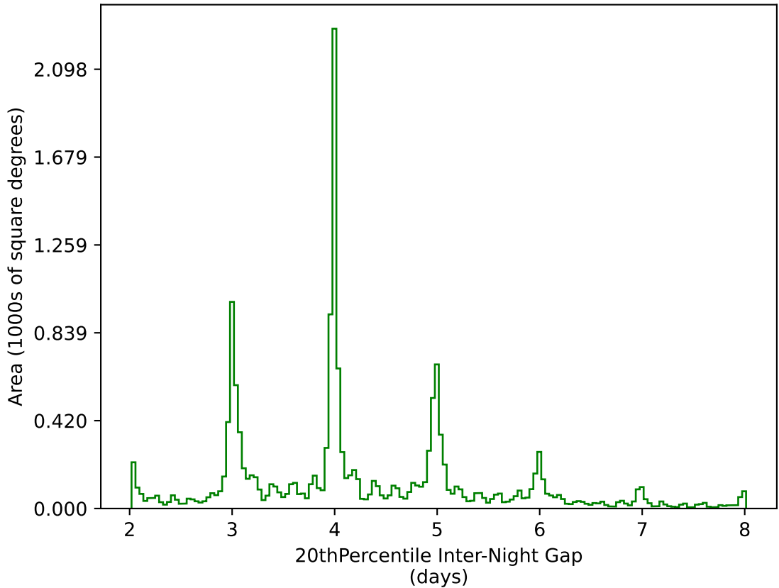
too_elab_r16_d2_gz_v3.4_10yrs WFD g band: 20thPercentile Inter-Night Gap
