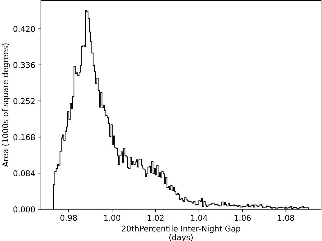
too_elab_r16_d2_gz_v3.4_10yrs WFD all bands: 20thPercentile Inter-Night Gap
