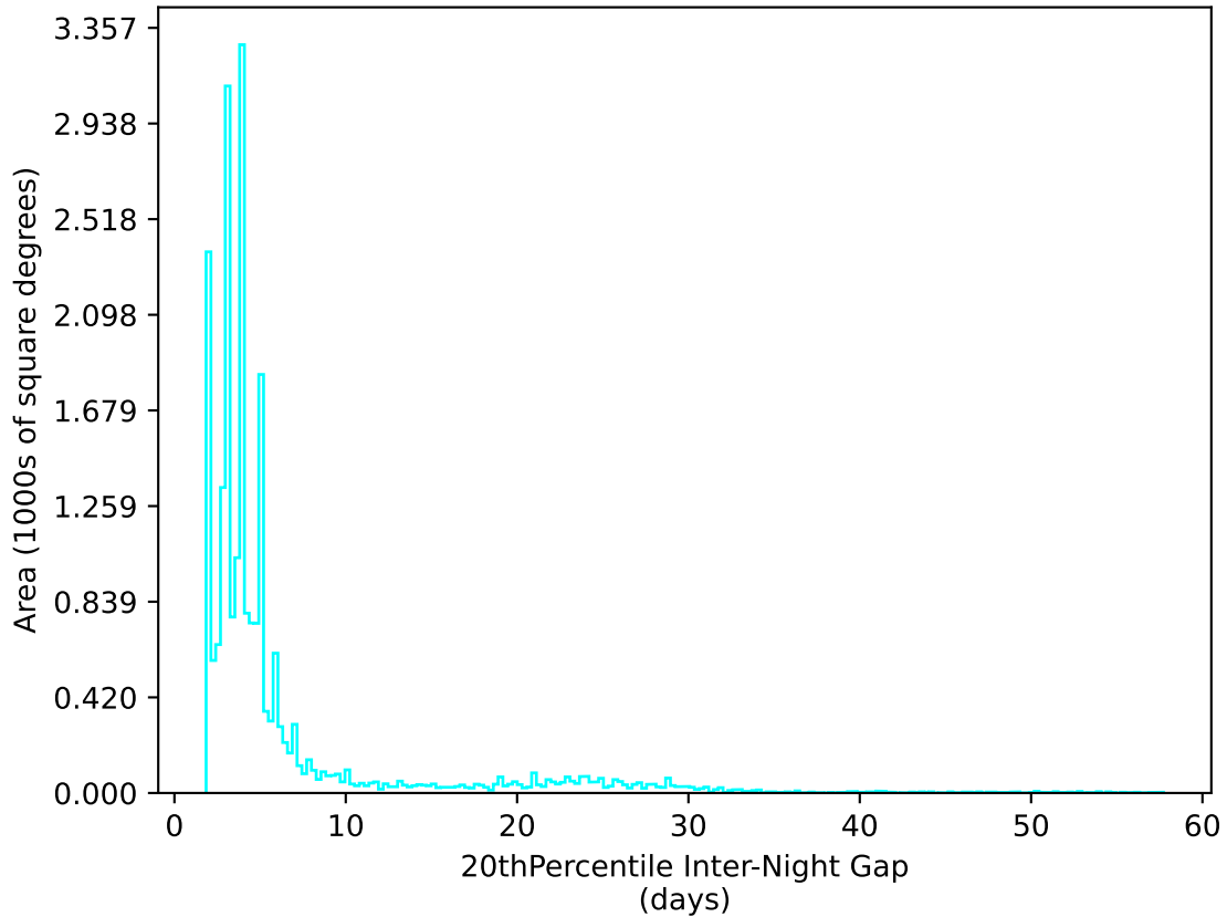
too_elab_r16_d2_gz_v3.4_10yrs All sky u band: 20thPercentile Inter-Night Gap
