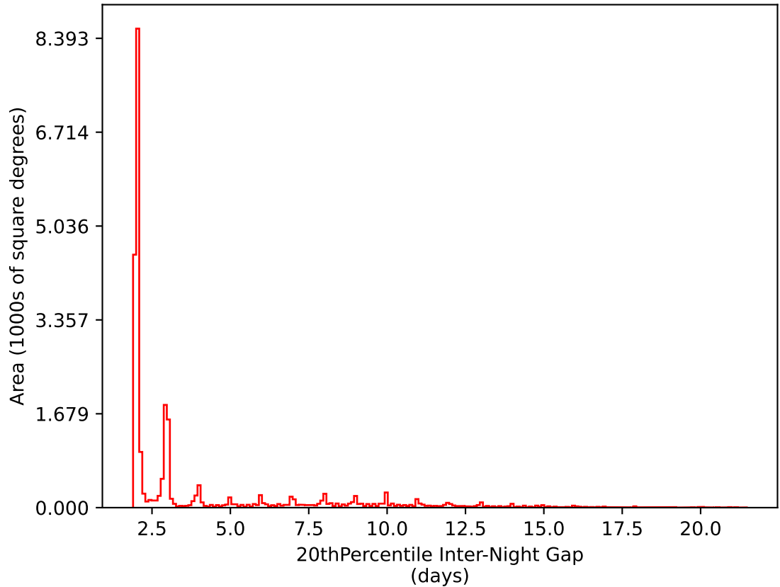
too_elab_r16_d2_gz_v3.4_10yrs All sky i band: 20thPercentile Inter-Night Gap
