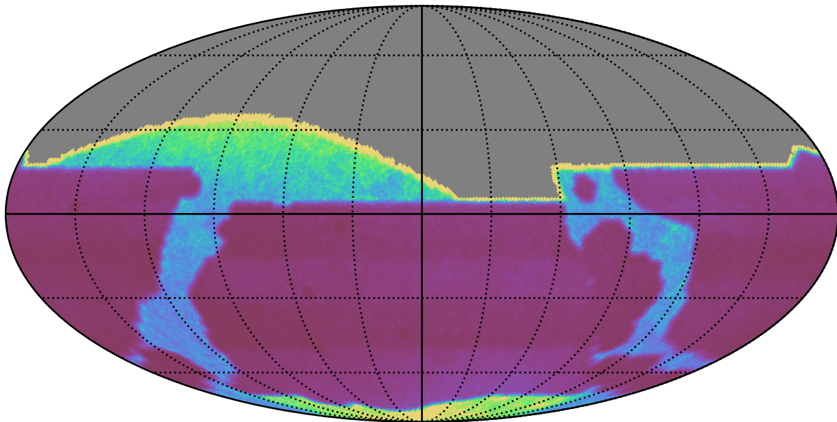
too_elab_r16_d2_gz_v3.4_10yrs : properMotion
