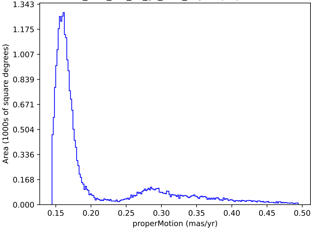
too_elab_r16_d2_gz_v3.4_10yrs : properMotion
