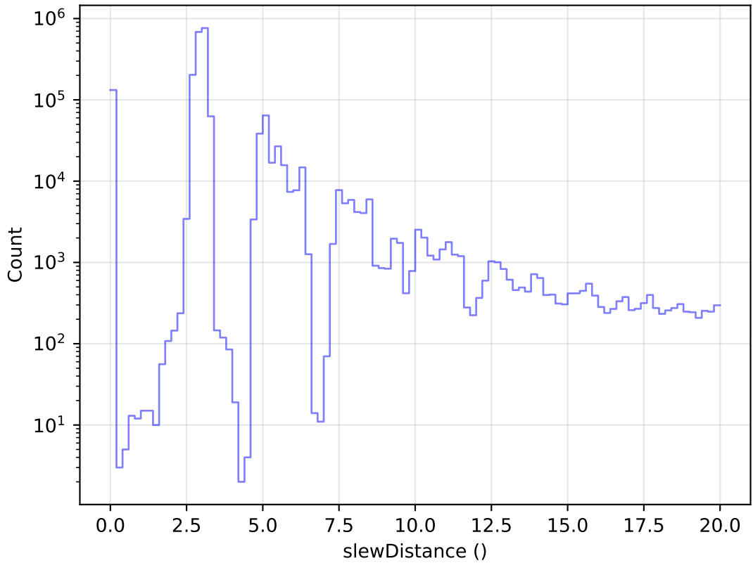
too_elab_r16_d2_gz_v3.4_10yrs All visits: Zoom Slew Distance Histogram
