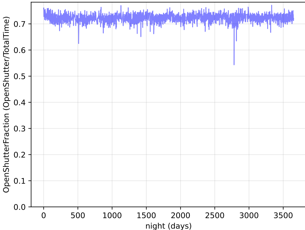
too_elab_r16_d2_gz_v3.4_10yrs : OpenShutterFraction
