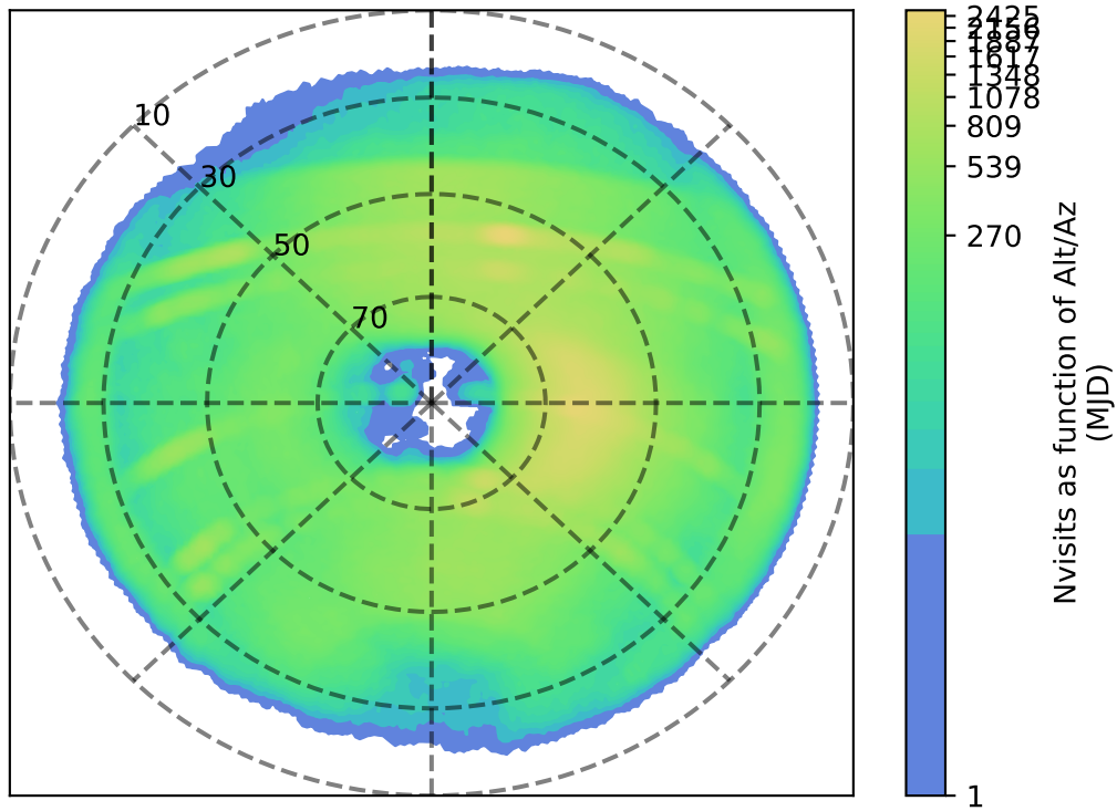
too_elab_r16_d2_gz_v3.4_10yrs z: Nvisits as function of Alt/Az
