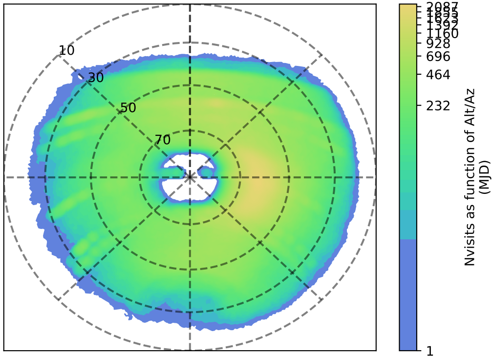
too_elab_r16_d2_gz_v3.4_10yrs y: Nvisits as function of Alt/Az
