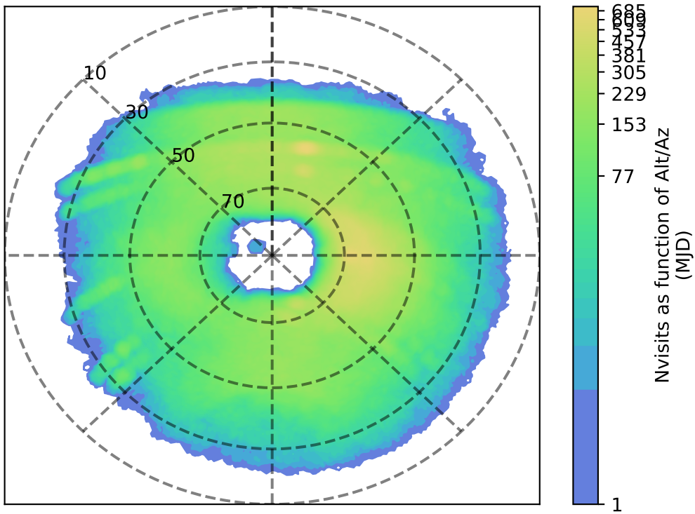
too_elab_r16_d2_gz_v3.4_10yrs u: Nvisits as function of Alt/Az
