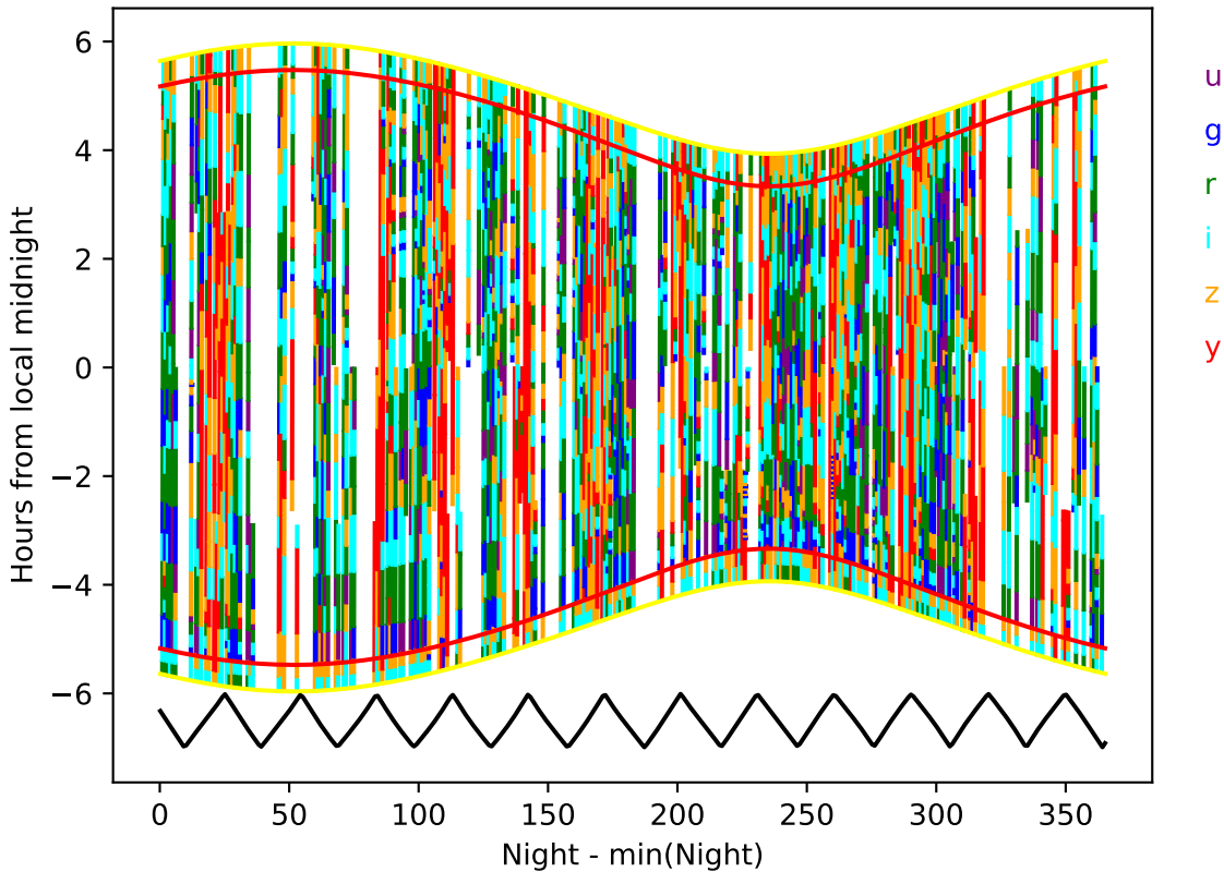
too_elab_r16_d2_gz_v3.4_10yrs year 7-8: Hourglass
