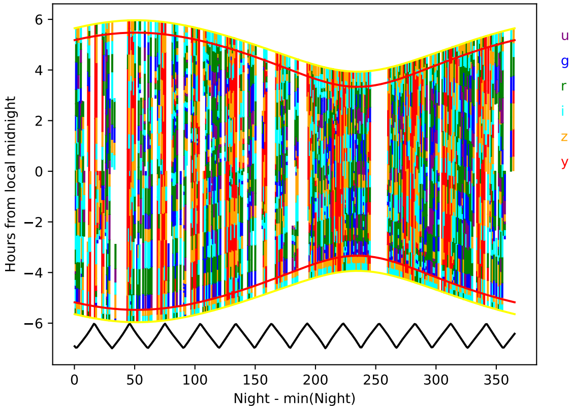
too_elab_r16_d2_gz_v3.4_10yrs year 5-6: Hourglass
