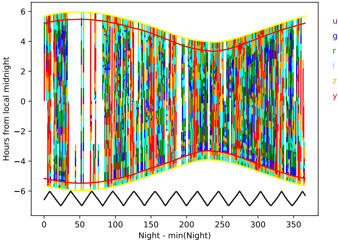
too_elab_r16_d2_gz_v3.4_10yrs year 3-4: Hourglass
