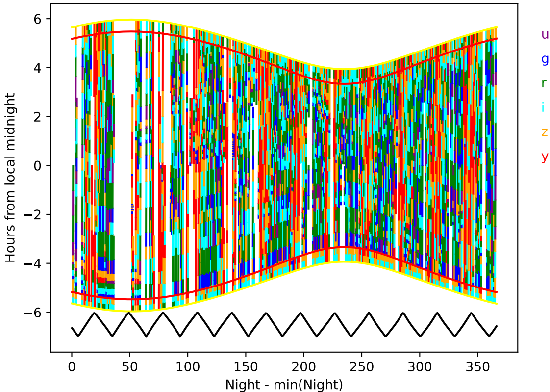
too_elab_r16_d2_gz_v3.4_10yrs year 2-3: Hourglass
