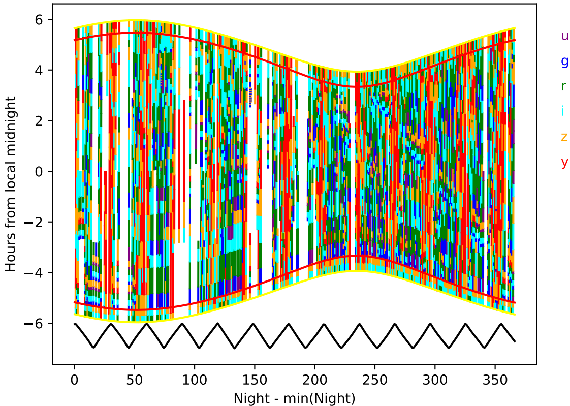
too_elab_r16_d2_gz_v3.4_10yrs year 1-2: Hourglass
