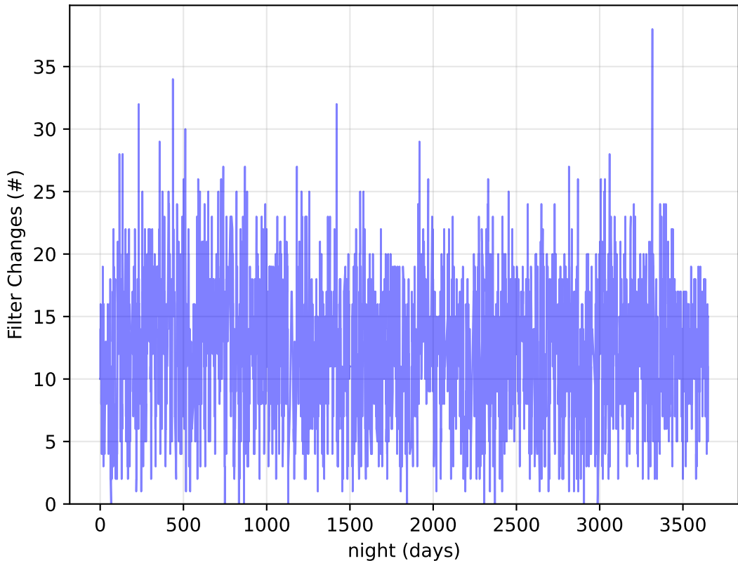
too_elab_r16_d2_gz_v3.4_10yrs : Filter Changes
