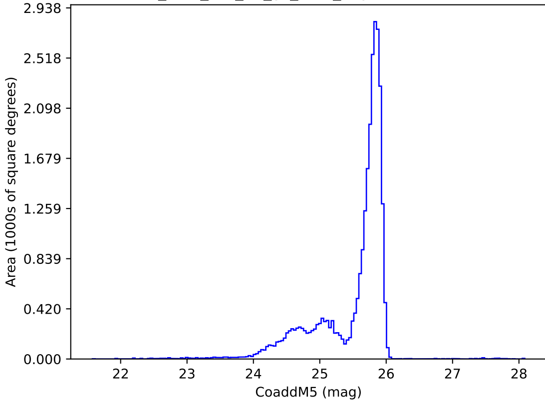
too_elab_r16_d2_gz_v3.4_10yrs z: CoaddM5
