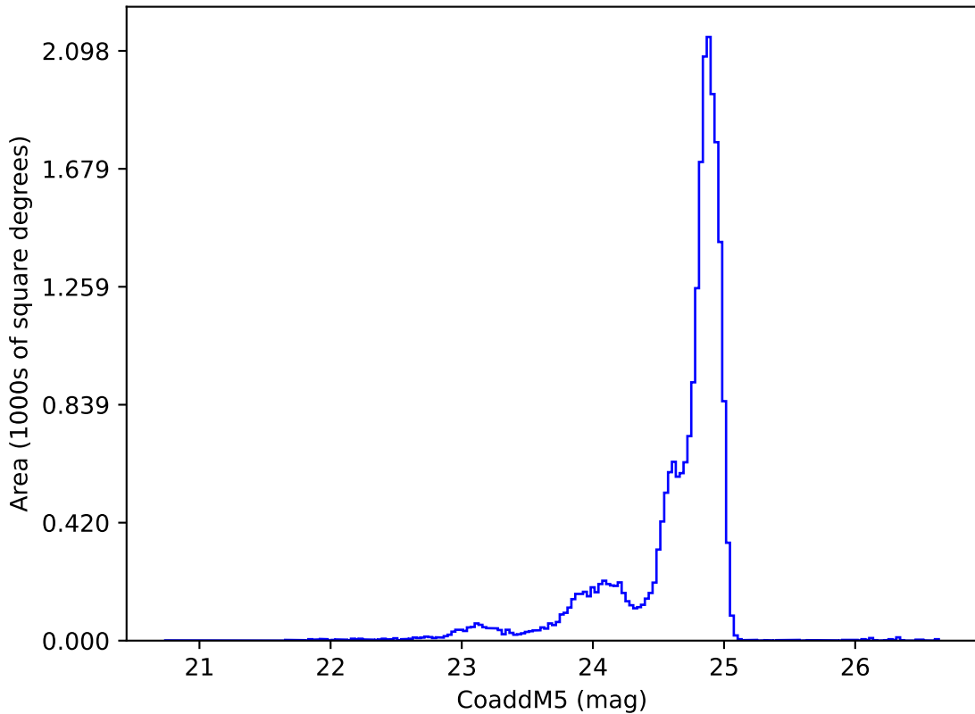
too_elab_r16_d2_gz_v3.4_10yrs y: CoaddM5
