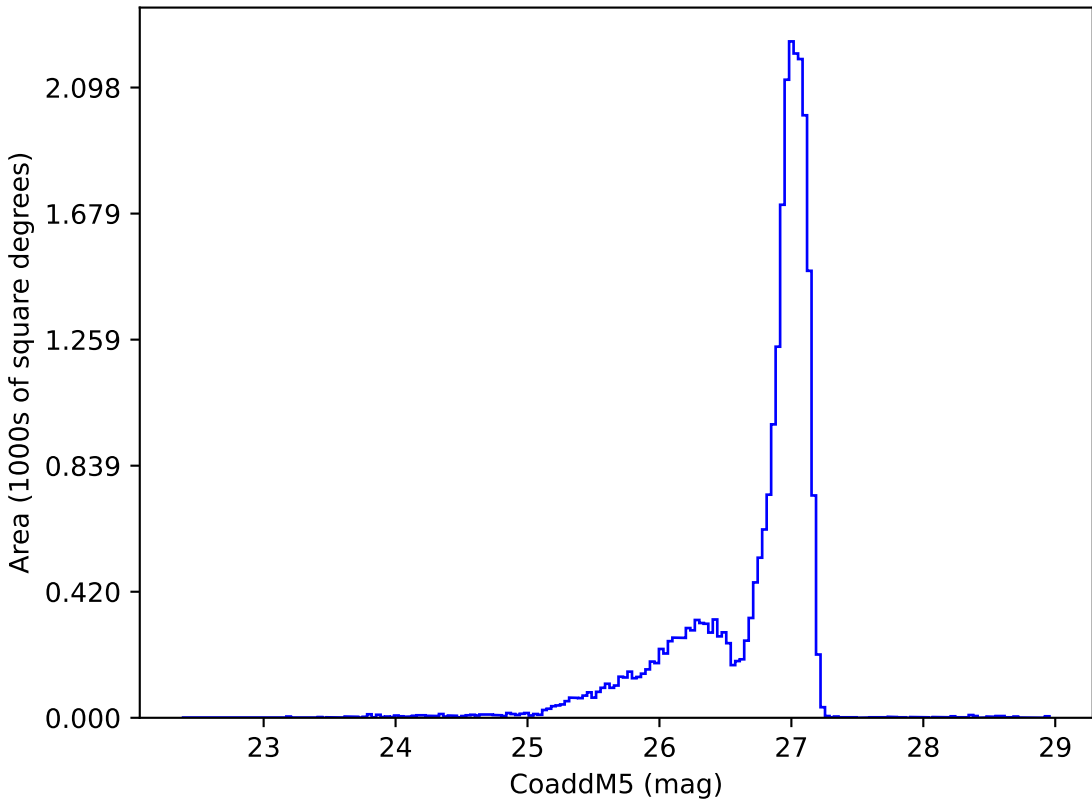
too_elab_r16_d2_gz_v3.4_10yrs r: CoaddM5
