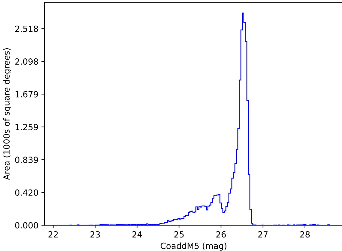
too_elab_r16_d2_gz_v3.4_10yrs i: CoaddM5
