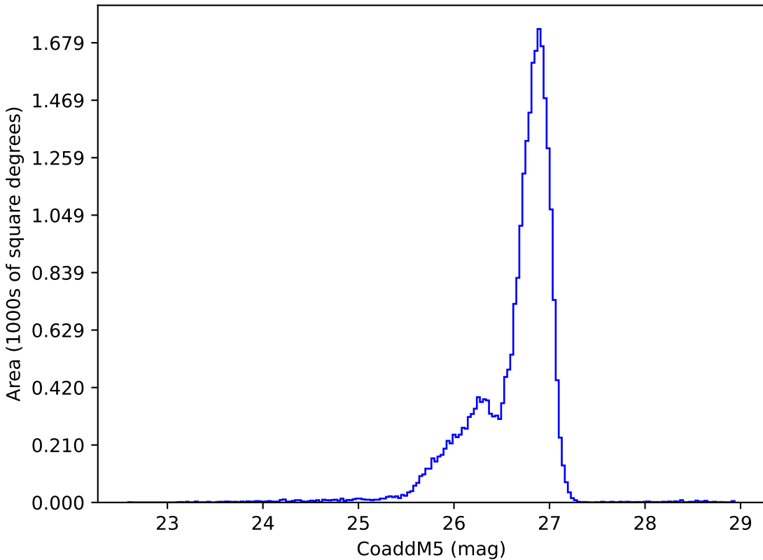
too_elab_r16_d2_gz_v3.4_10yrs g: CoaddM5
