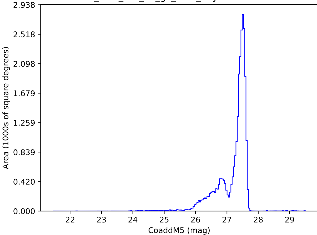
too_elab_r16_d2_gz_v3.4_10yrs : CoaddM5
