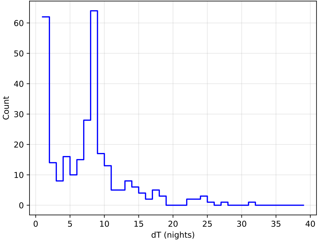
too_elab_r16_d2_gz_v3.4_10yrs all bands: DD:XMM_LSS Delta Nights Histogram
