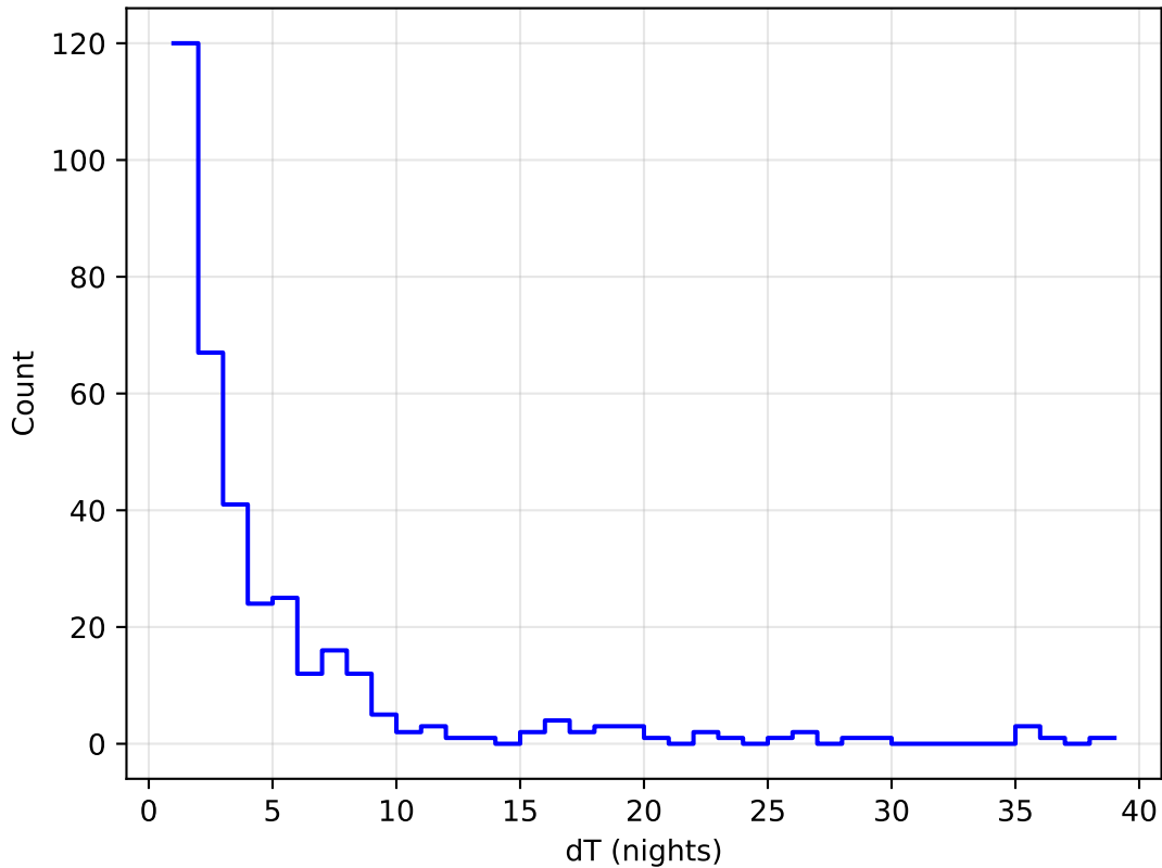
too_elab_r16_d2_gz_v3.4_10yrs all bands: DD:WFD Delta Nights Histogram
