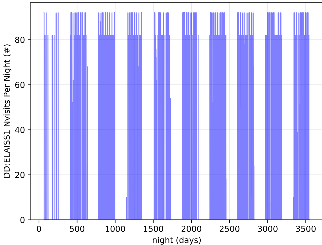
too_elab_r16_d2_gz_v3.4_10yrs all bands: DD:ELAISS1 Nvisits Per Night
