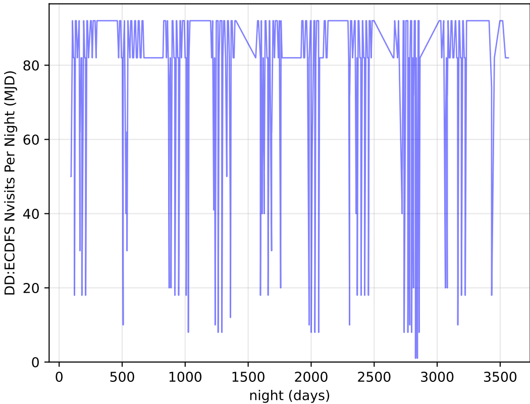
too_elab_r16_d2_gz_v3.4_10yrs all bands: DD:ECDFS Nvisits Per Night
