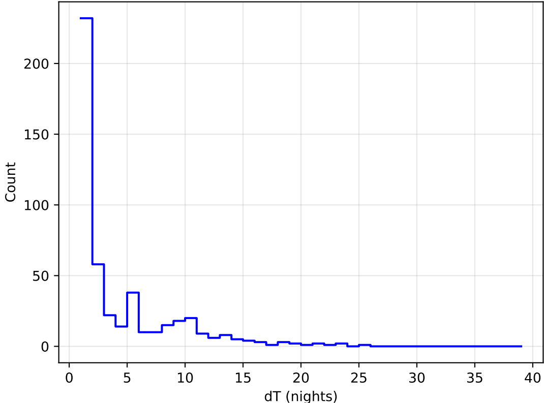
too_elab_r16_d2_gz_v3.4_10yrs all bands: DD: COSMOS Delta Nights Histogram
