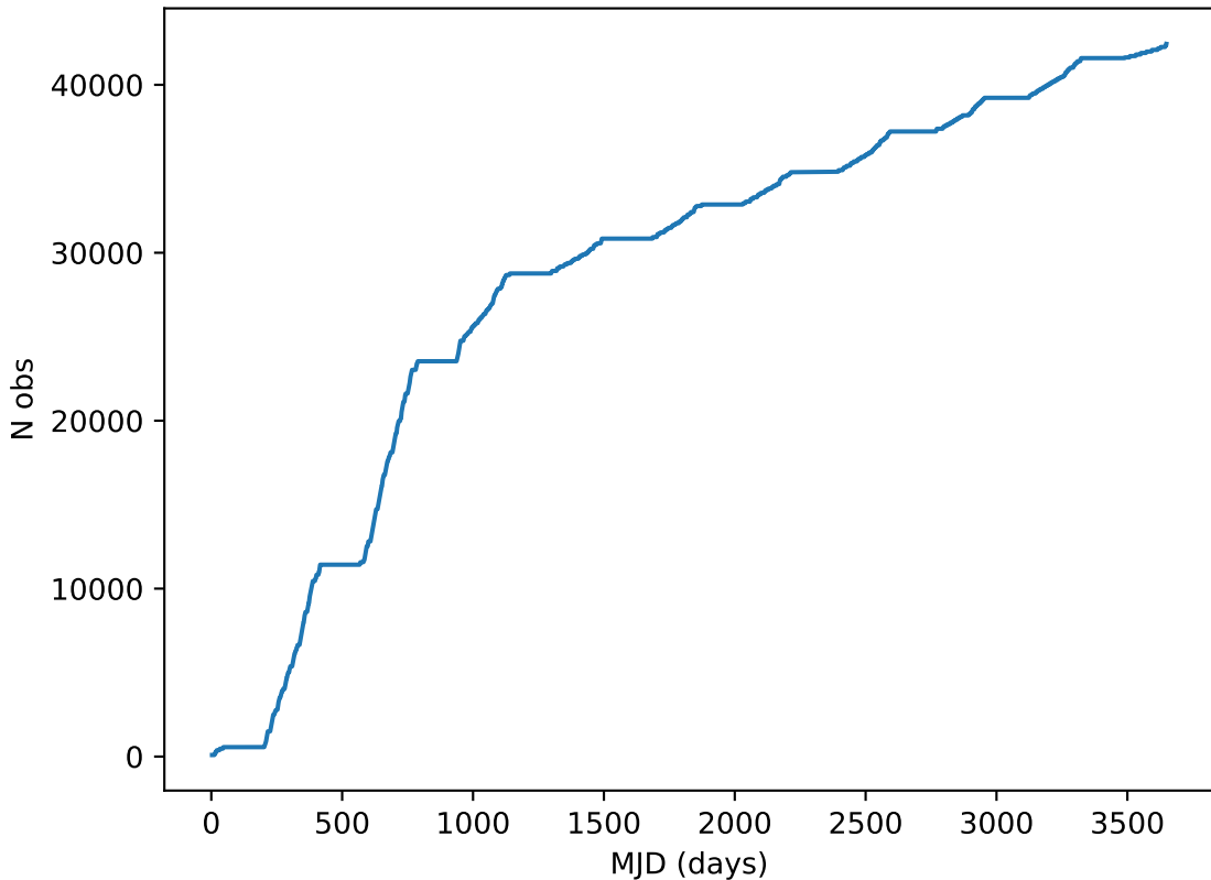
too_elab_r16_d2_gz_v3.4_10yrs all bands: DD: COSMOS Cumulative NVisits
