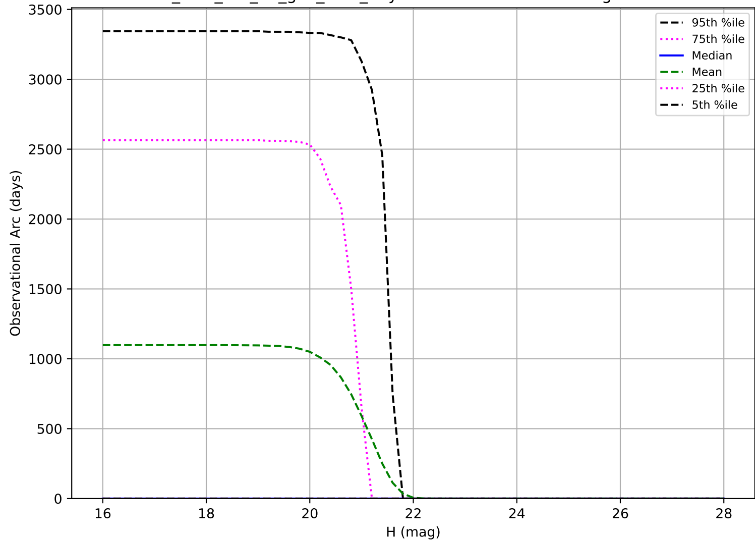
too_elab_r16_d2_griz_v3.4_10yrs: Observational Arc Length Vatira
