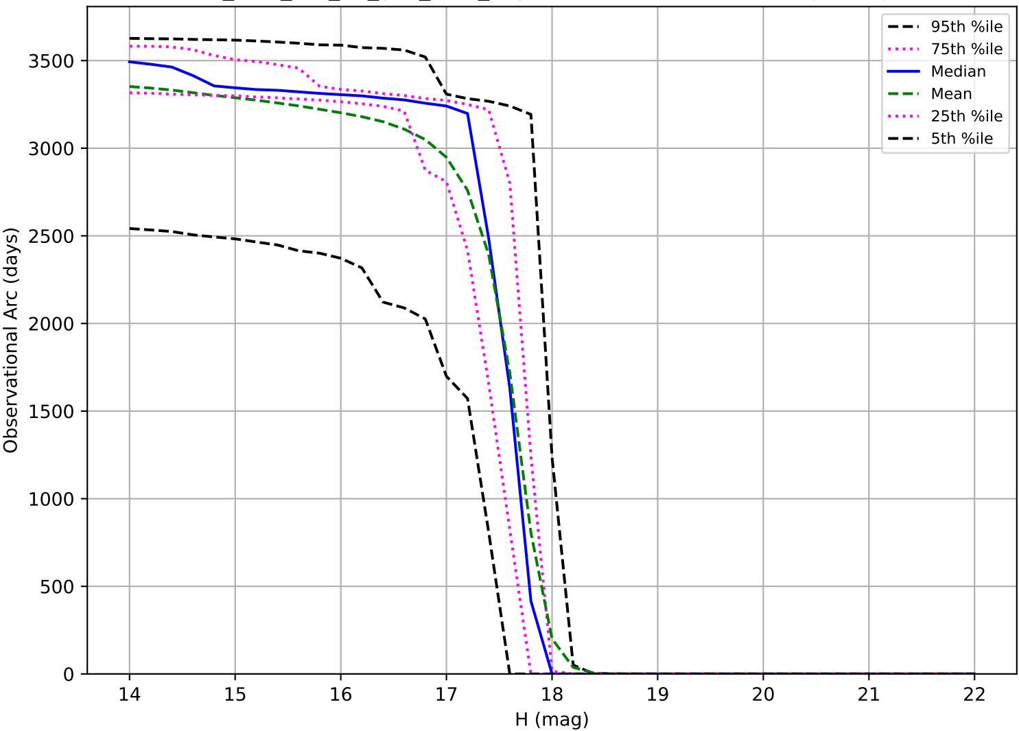
too_elab_r16_d2_griz_v3.4_10yrs: Observational Arc Length Trojan
