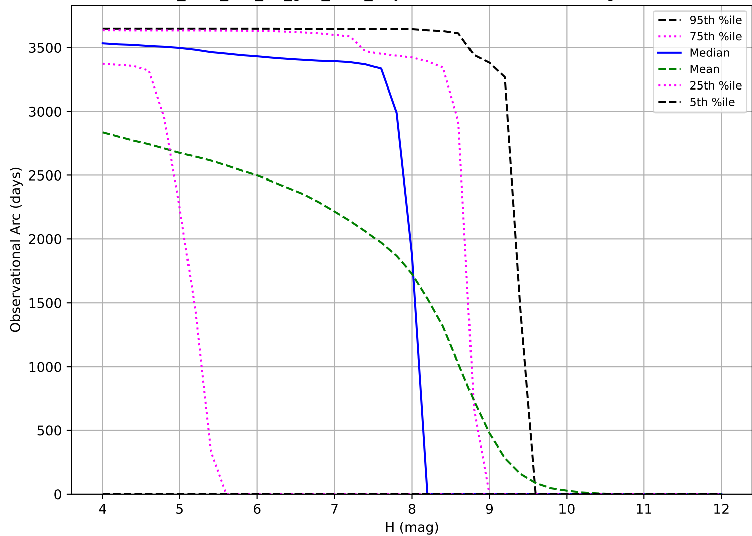
too_elab_r16_d2_griz_v3.4_10yrs: Observational Arc Length TNO
