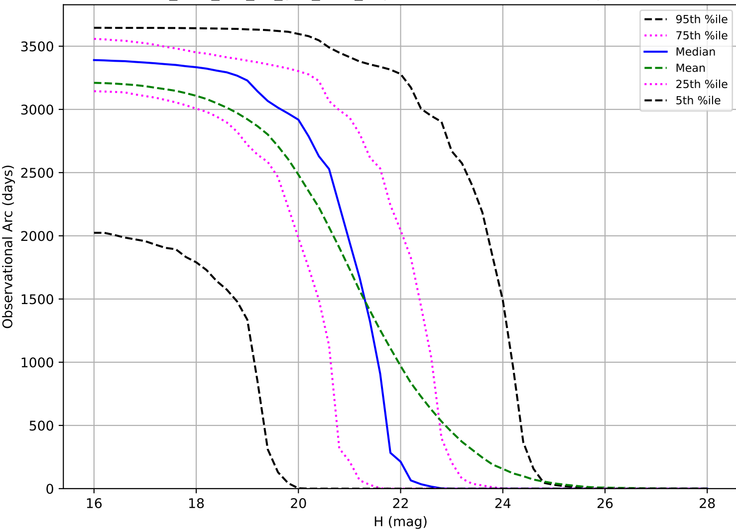
too_elab_r16_d2_griz_v3.4_10yrs: Observational Arc Length PHA
