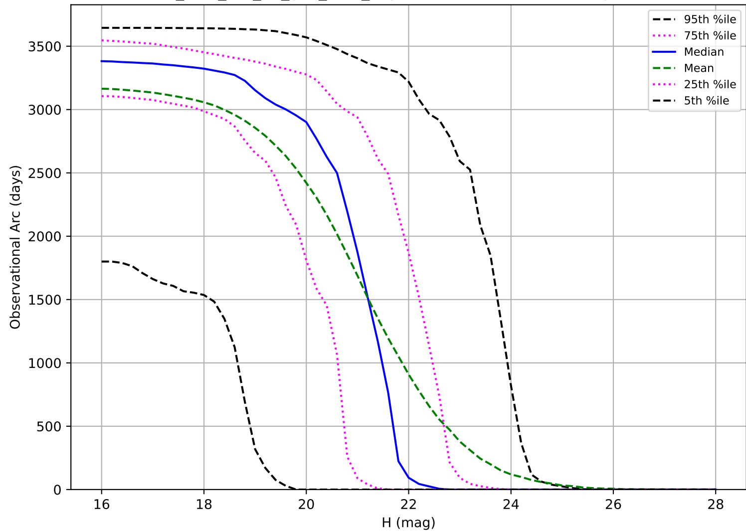
too_elab_r16_d2_griz_v3.4_10yrs: Observational Arc Length NEO
