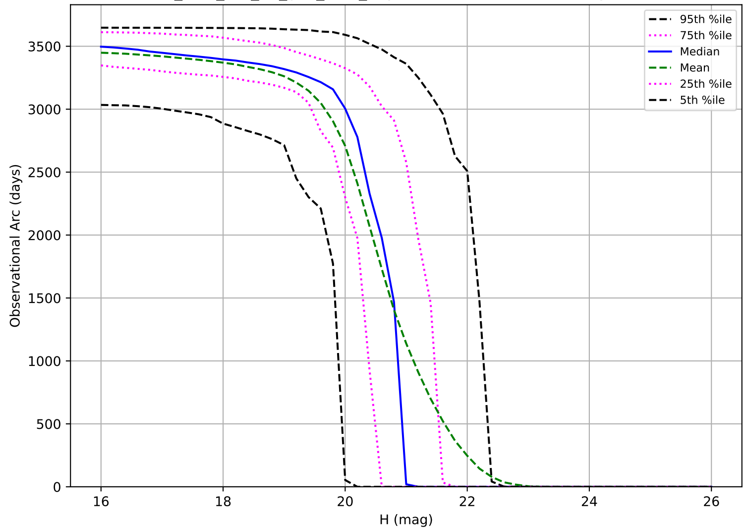
too_elab_r16_d2_griz_v3.4_10yrs: Observational Arc Length MBA
