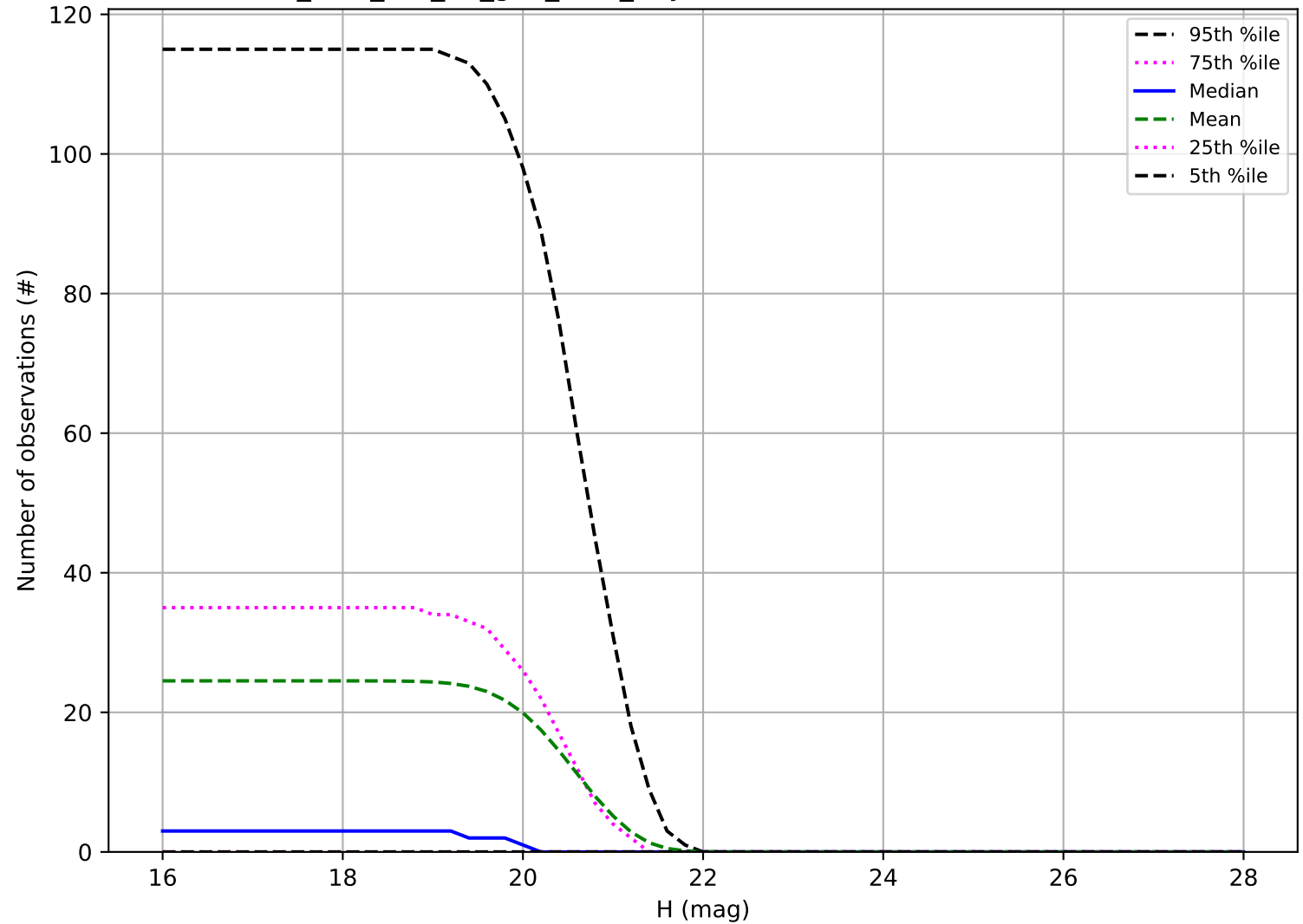
too_elab_r16_d2_griz_v3.4_10yrs: Number of observations Vatira
