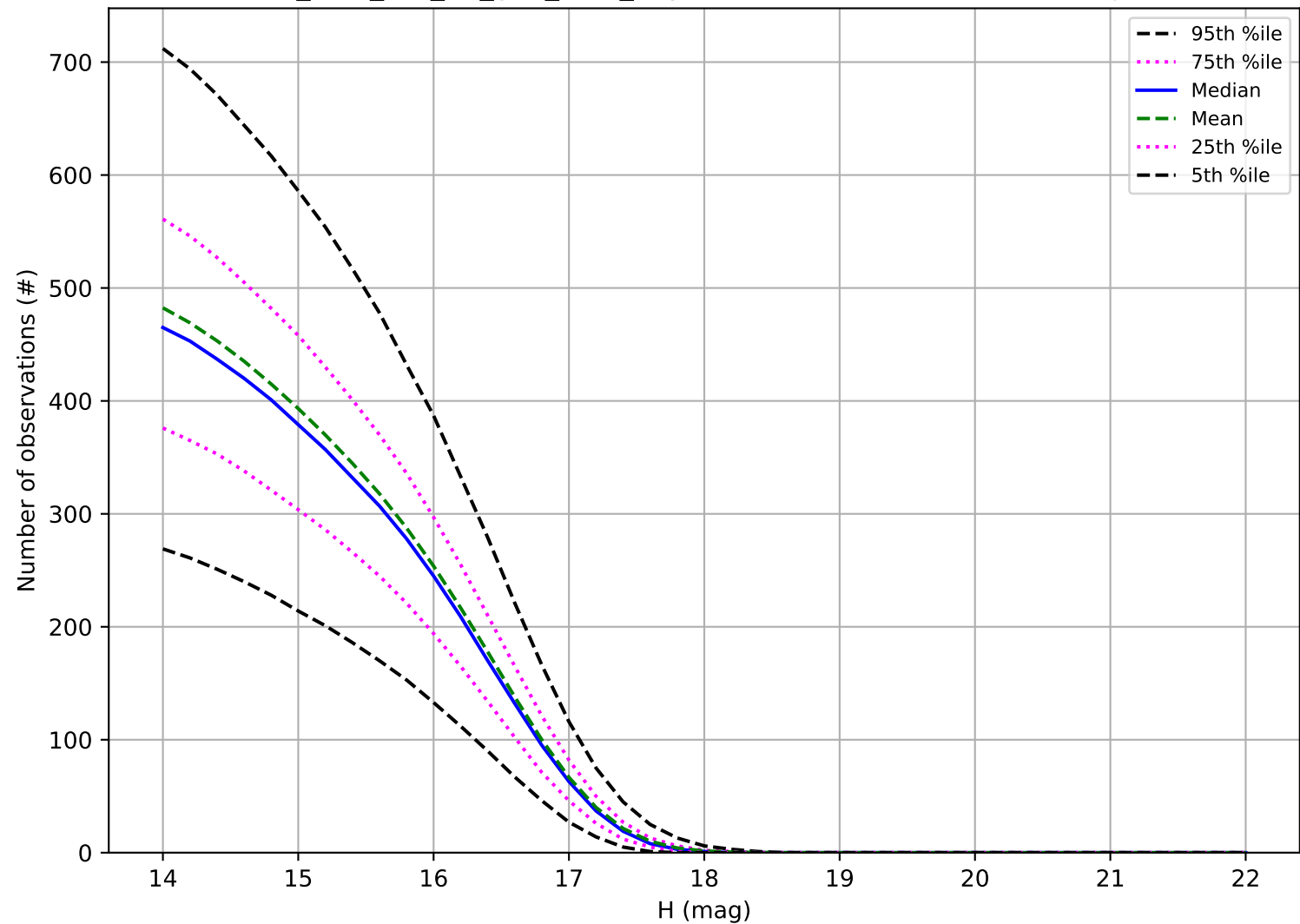
too_elab_r16_d2_griz_v3.4_10yrs: Number of observations Trojan
