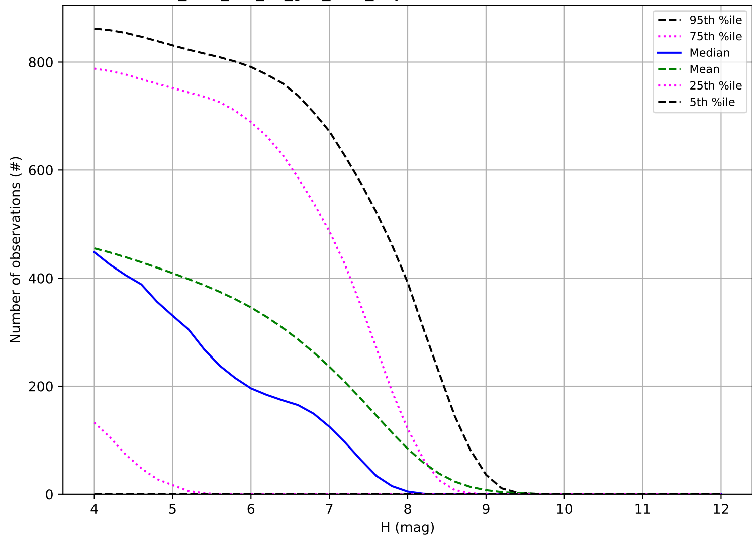
too_elab_r16_d2_griz_v3.4_10yrs: Number of observations TNO
