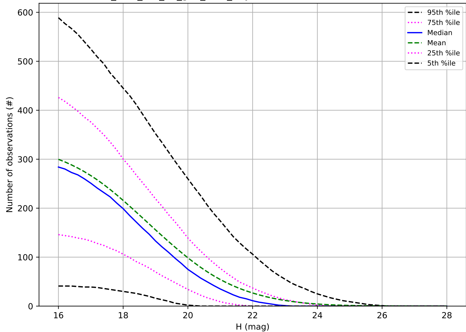
too_elab_r16_d2_griz_v3.4_10yrs: Number of observations PHA
